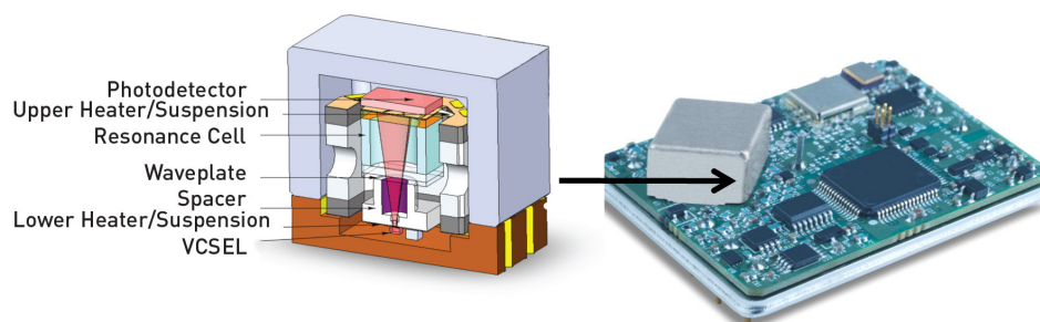
Figure 1. SA.45s physics package. The cutaway drawing on the left shows the leadless chip carrier, used to mount the physics package to the printed circuit board, in brown, and the ceramic cap which maintains the vacuum around the physics package, in gray. The photo on the right shows the physics package mounted to the printed circuit board and covered with a layer of mu-metal shielding.
